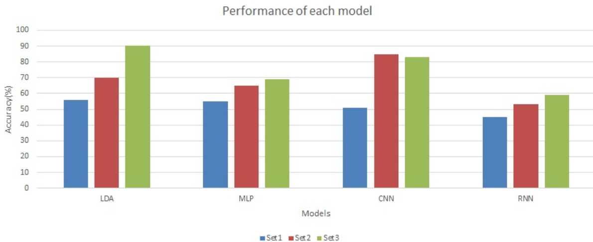
Figure 5.1: This graph plots the accuracy attained by each model w.r.t each of the inputs data set
