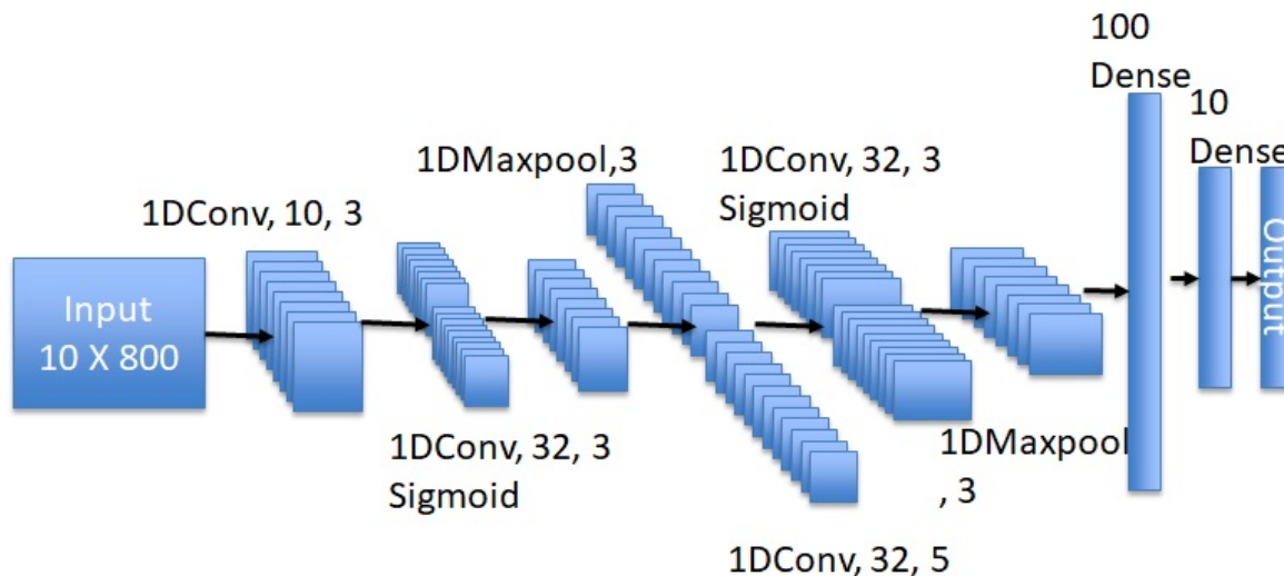
Figure 4.3: CNN structure
