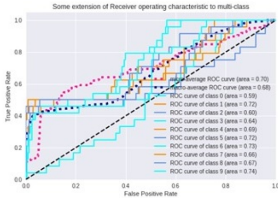
((a)) ROC of Style 1 batch
